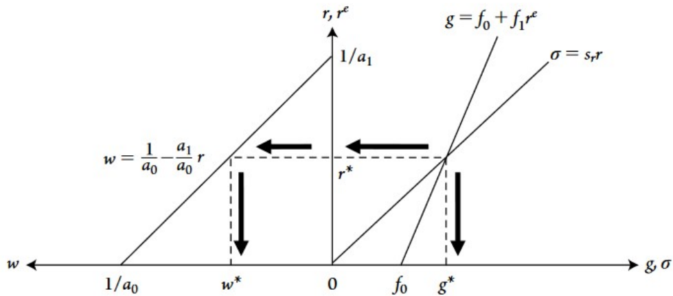
Figure 6.3: Neo-robinsonian model
